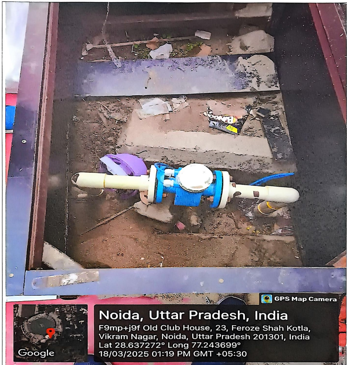
Water flow Meter (Tubewell no.2)
